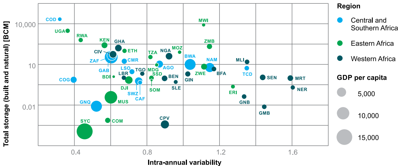
Figure 6. Total surface water storage in billion cubic metres (BCM) versus intra-annual rainfall variability for sub-Saharan Africa countries
